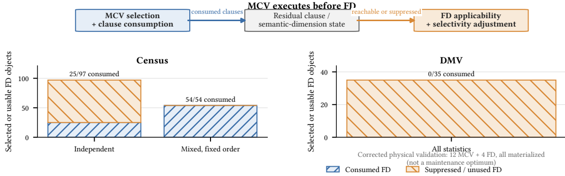
Figure 3: Directed MCV-to-FD composition and FD consumption. MCV clause consumption feeds FD residual state. Census independent mechanism selection chooses 97 FDs, 72 unused after composition, whereas fixed-precedence mixed selection chooses 54, all consumed. In corrected DMV, the all-statistics state consumes zero of 35 usable FDs; the corrected physical validation state contains 12 MCV and four FD objects. The latter is semantic validation, not a maintenance-constrained optimum.
