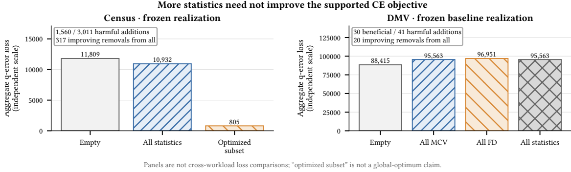
Figure 2: Cross-workload non-monotonicity. Separate, independently scaled panels compare empty and complete states. Census has 1,444 beneficial, seven neutral, and 1,560 harmful singleton additions among 3,011 candidates, plus 317 improving removals. Corrected DMV has 30 beneficial and 41 harmful additions among 71 candidates, plus 20 improving removals. This is contextual evidence from two frozen payload realizations, not a universal workload property.
