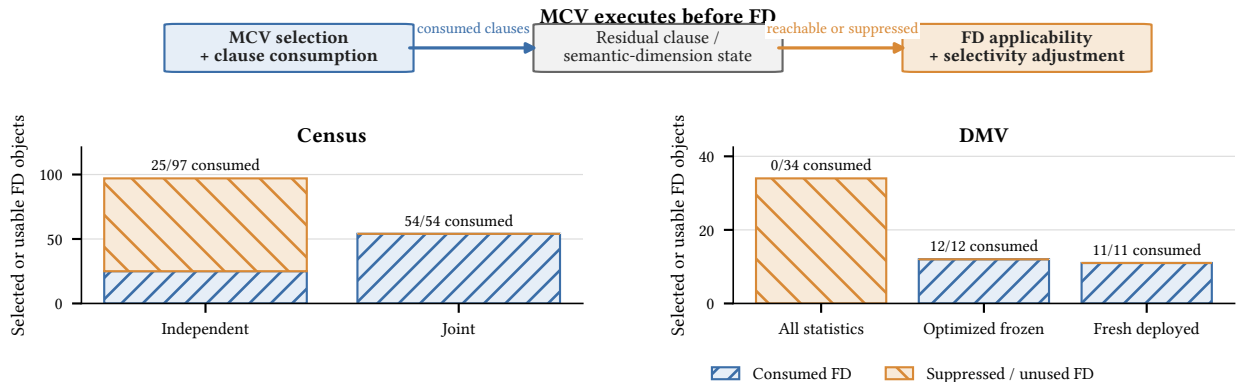
Figure 4: Directed MCV-to-FD composition and FD consumption. MCV clause consumption feeds FD residual state. Census independent optimization selects 97 FDs, 72 unused after composition; joint optimization selects 54, all consumed. DMV all-statistics consumes zero of 34 usable FDs; optimization consumes all 12 selected frozen FDs and all 11 materialized fresh FDs.
