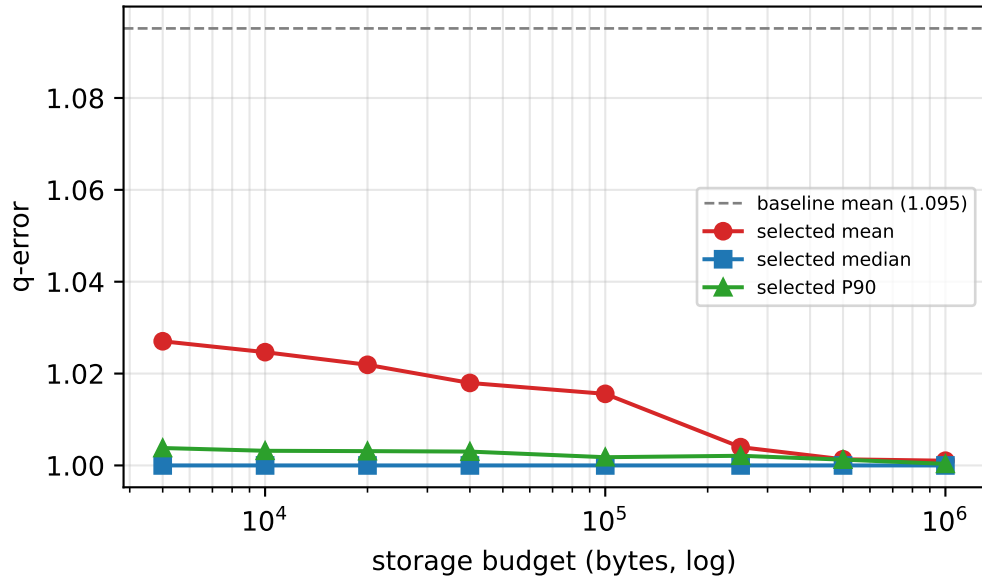
Budget-quality curve (multi-metric)
