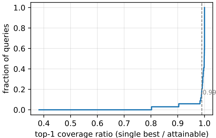
Single-statistic coverage (RQ2)
