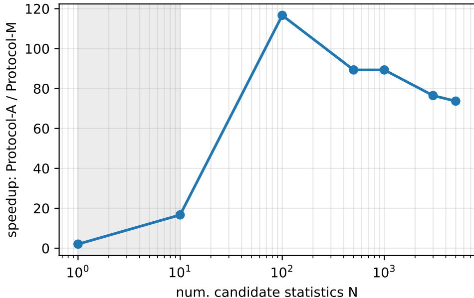
Catalog-mask speedup (wide synthetic table, target 1000)
