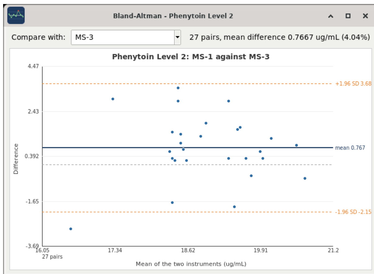
Figure 11: Bland-Altman
