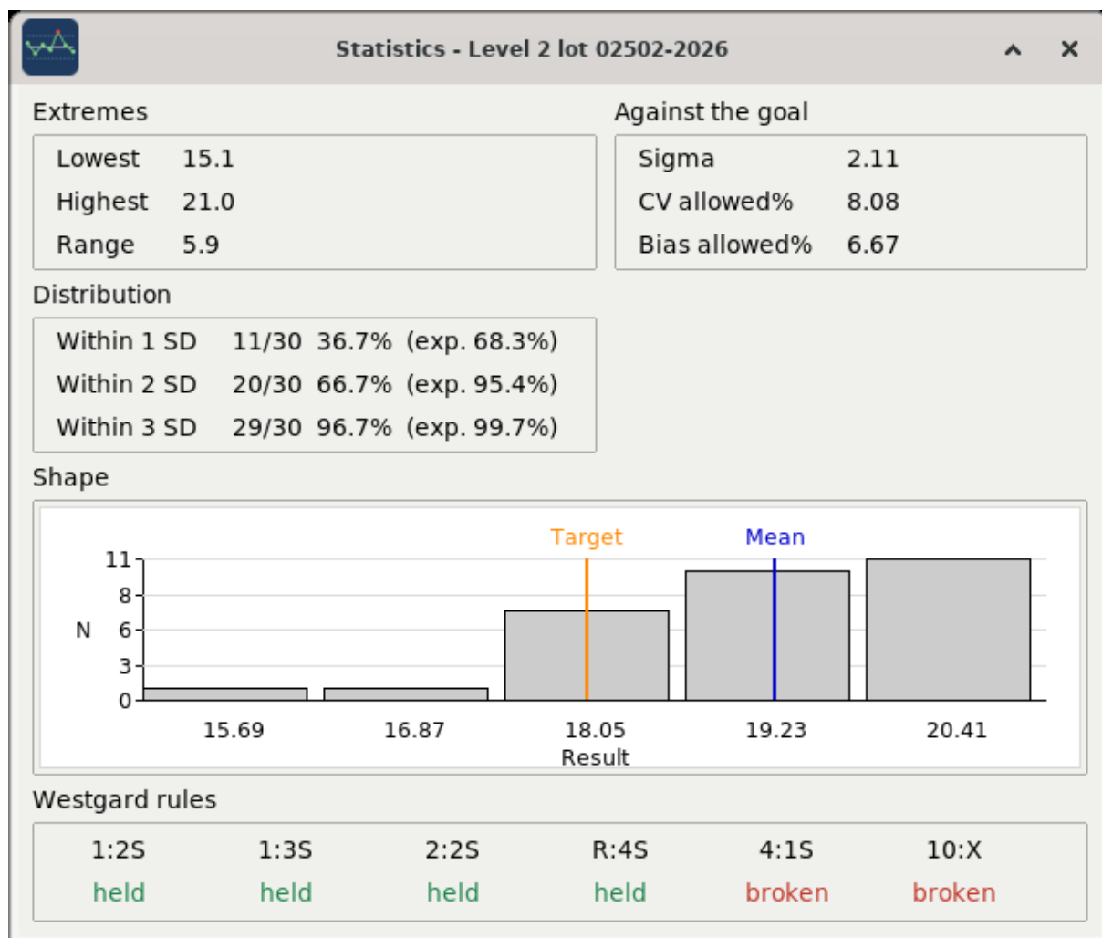
Figure 7: The statistics
