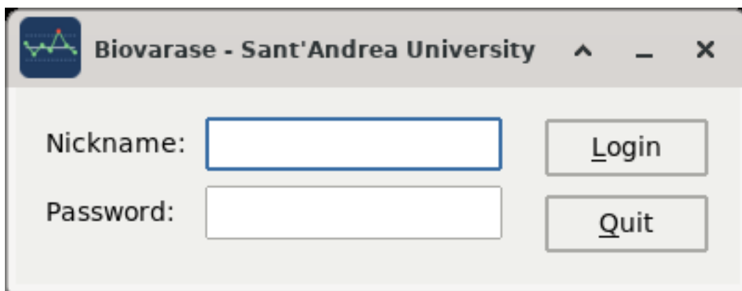
Figure 1: The login
