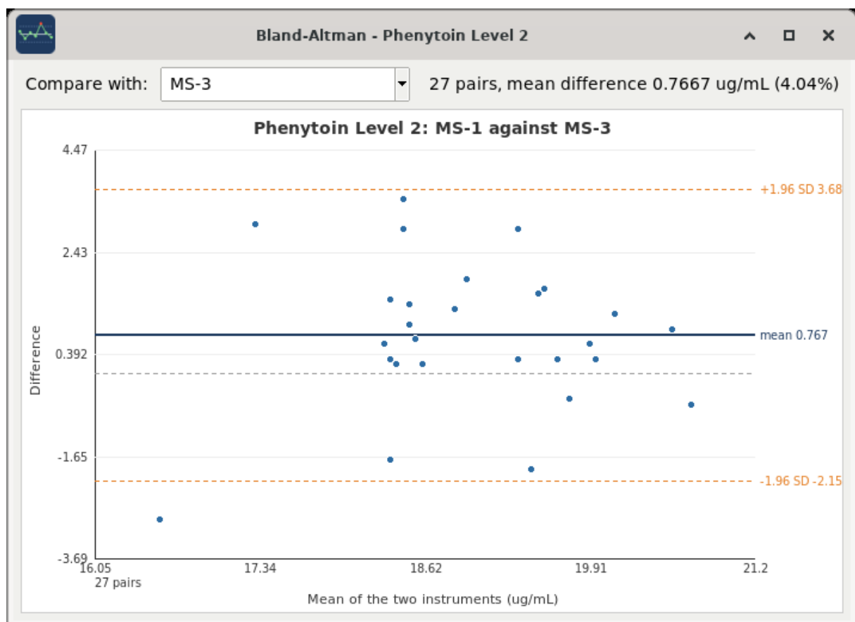
Figure 11: Bland-Altman
