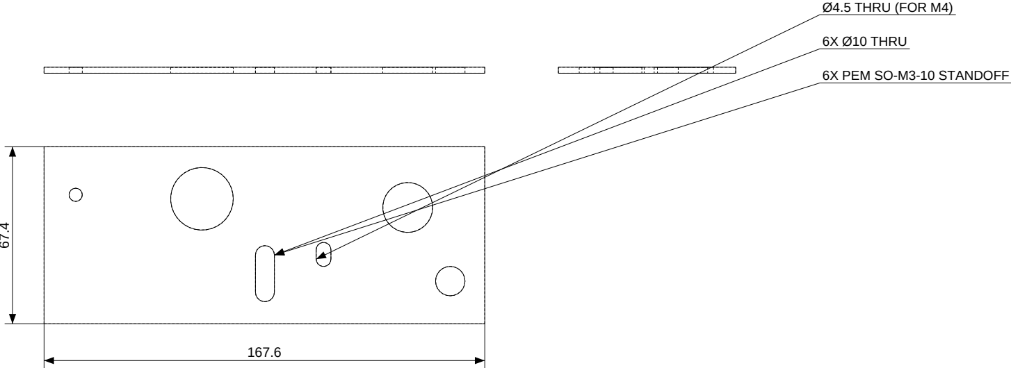
FLAT PATTERN (REF.)
