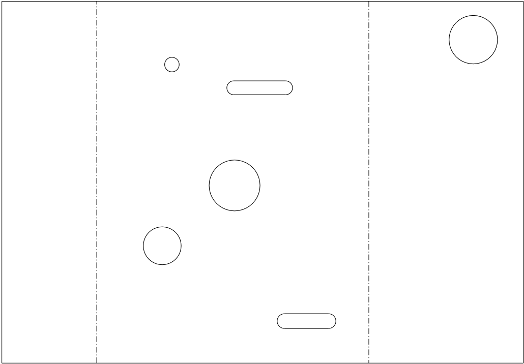
FLAT PATTERN (REF.)
