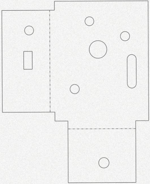
FLAT PATTERN (REF.)
