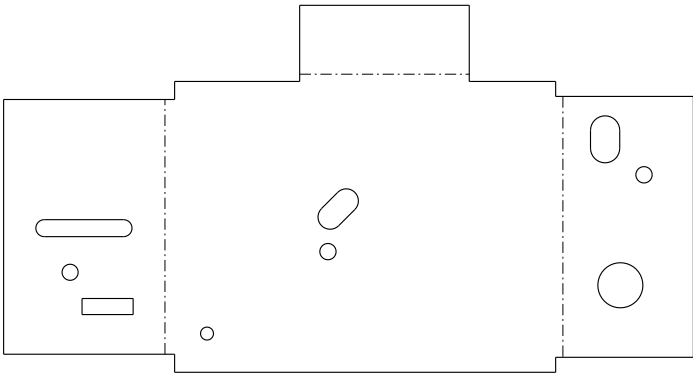
FLAT PATTERN (REF.)
