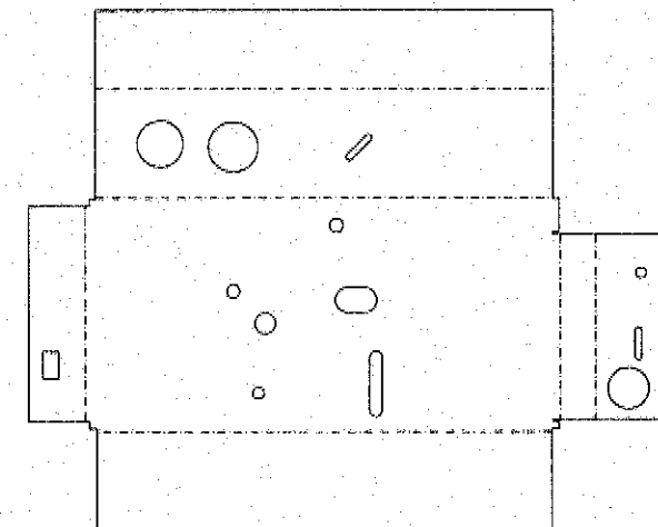
FLAT PATTERN (REF.)
