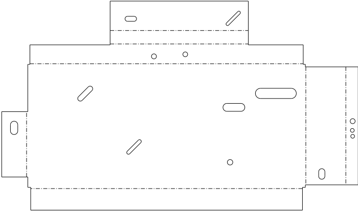
FLAT PATTERN (REF.)
