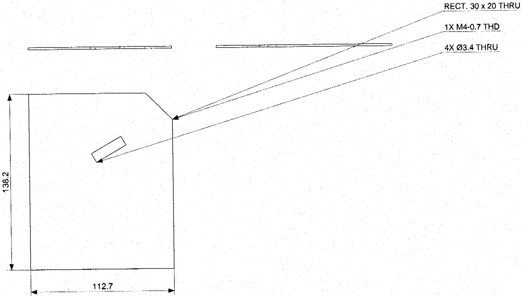
FLAT PATTERN (REF.)
