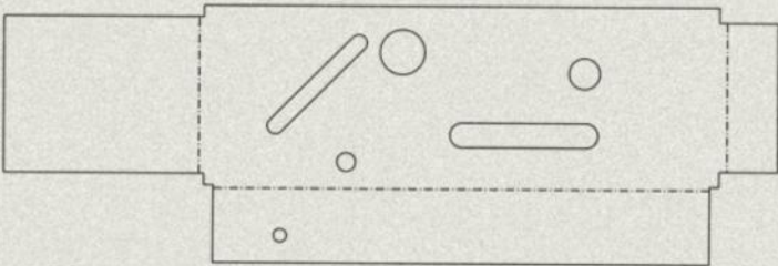
FLAT PATTERN (REF.)
