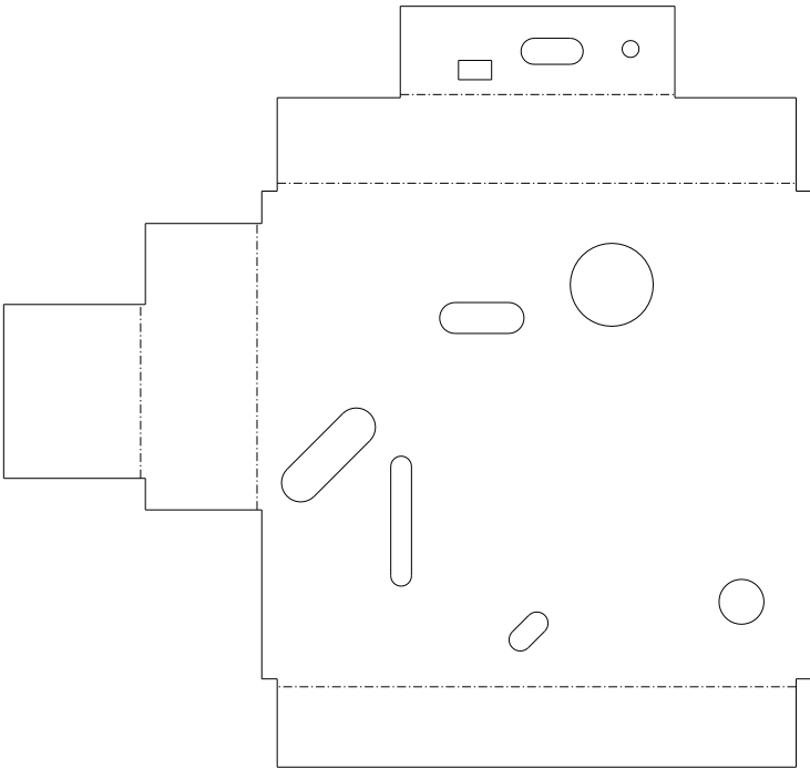
FLAT PATTERN (REF.)
