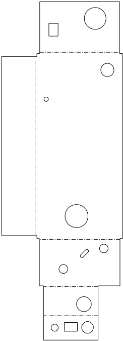
FLAT PATTERN (REF.)
