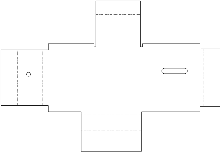
FLAT PATTERN (REF.)
