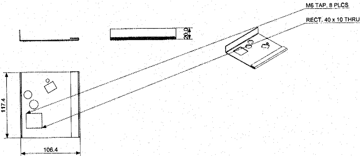
FLAT PATTERN (REF.)
