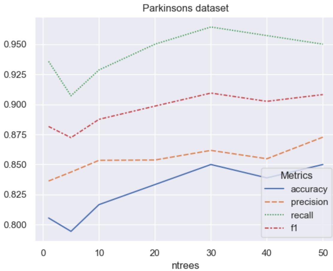
Figure 4: Parkinsons Accuracy and F1 Score Distribution
