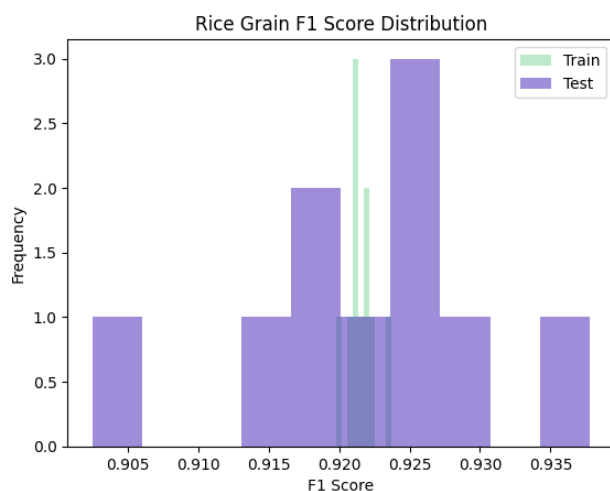
Figure 7: Rice F1 Score Distribution
