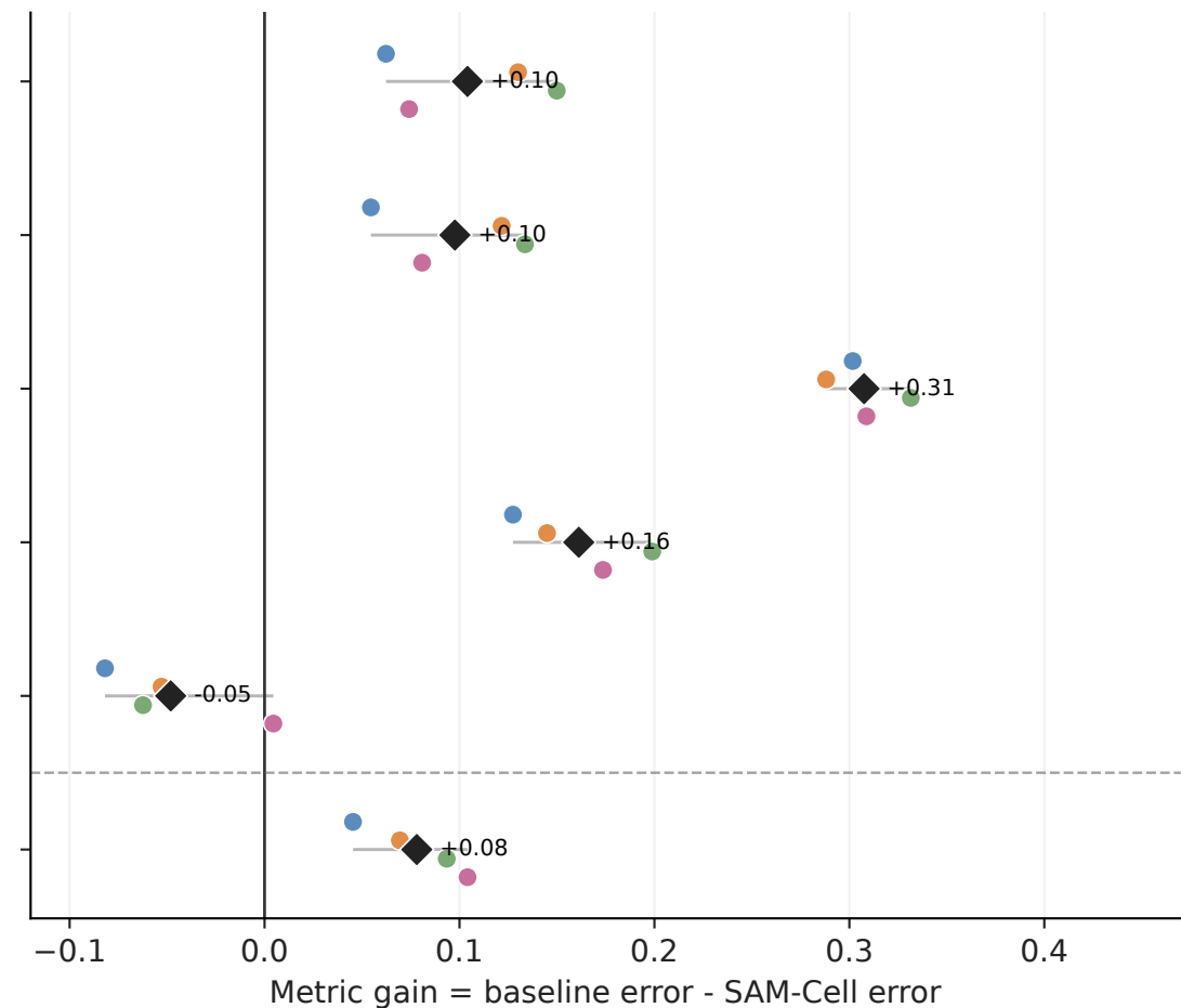
Error reduction vs CellSAM
