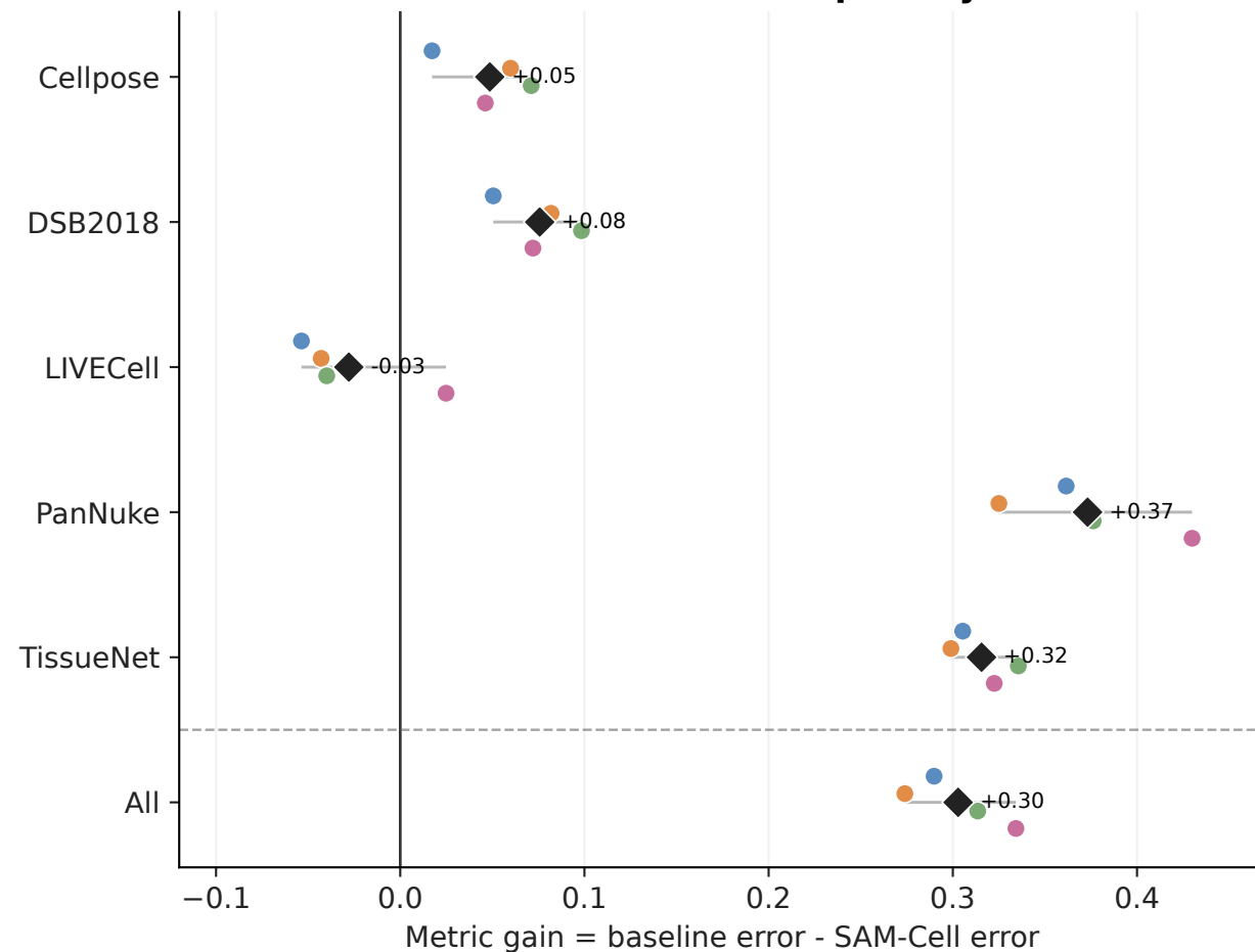
Error reduction vs Cellpose cyto3
