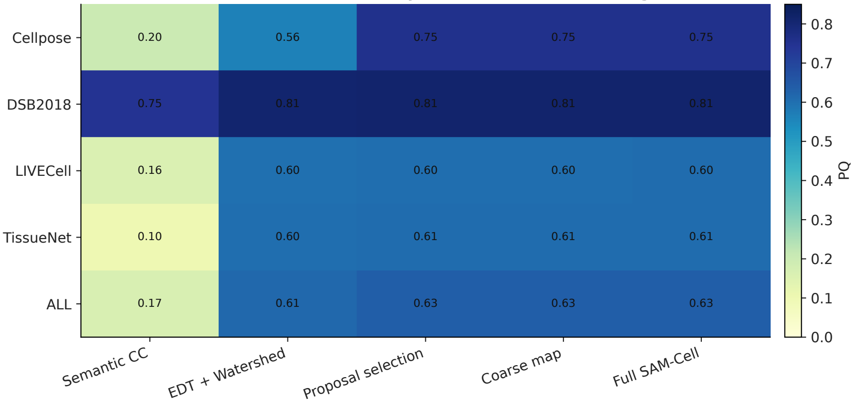
Far-OOD PQ heatmap by source and module stage
