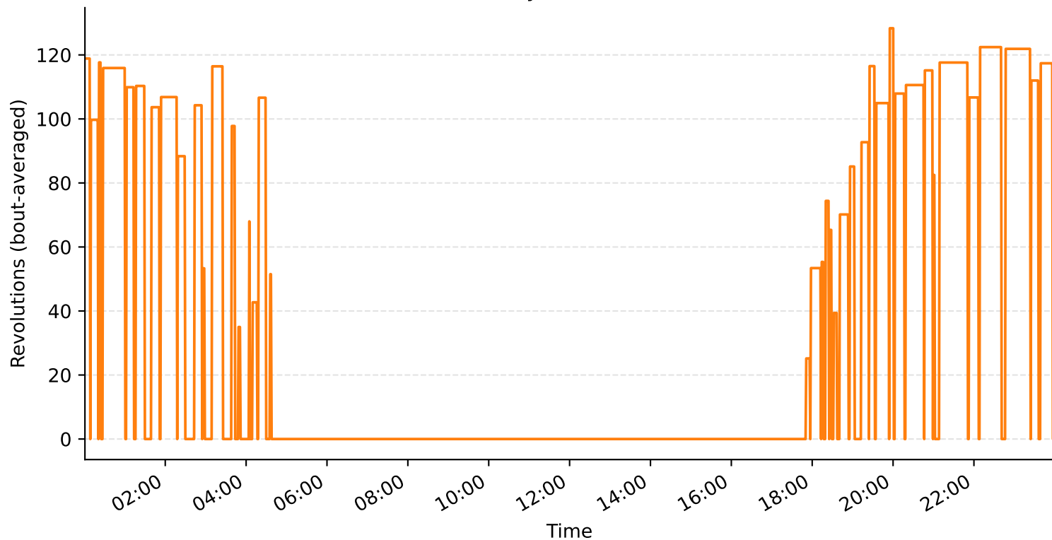
Cohort 1 - D16 - Bout Activity - LM45(SNr-DTA) ( \geq 10 revs/min)
