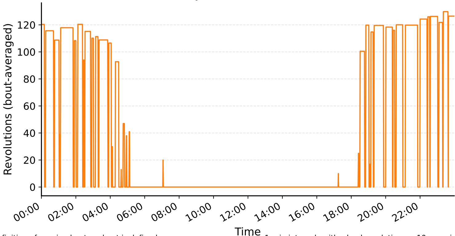
D5 - Bout Activity - SC15(Control) ( \geq 10 revs/min)
