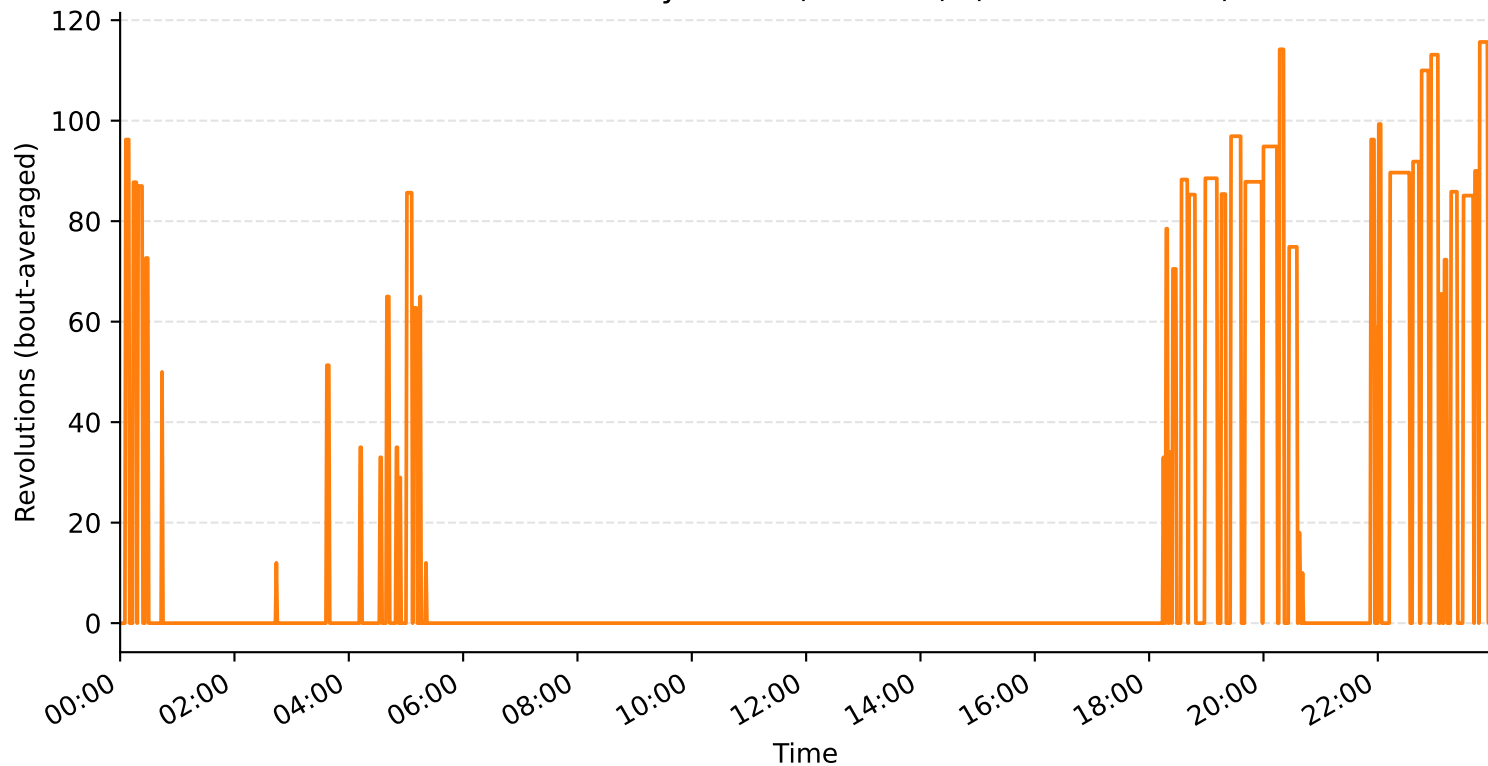
D12 - Bout Activity - SC04(SNr-DTA) ( \geq 10 revs/min)
