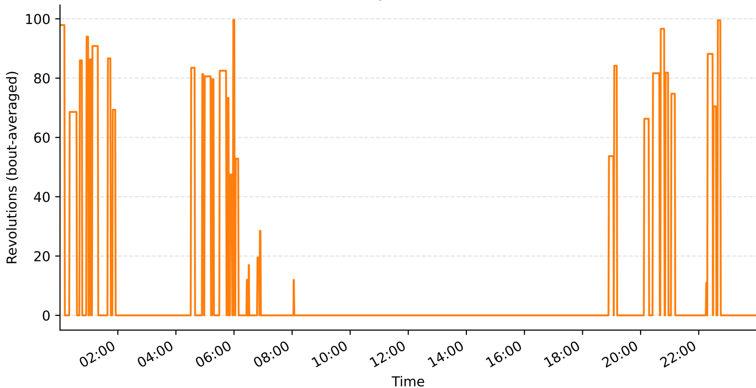
Cohort 4 - D13 - Bout Activity - SC32(SNr-DTA) ( \geq 10 revs/min)
