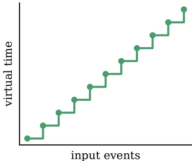
virtual clock
