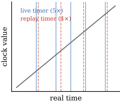
wall-clock time
