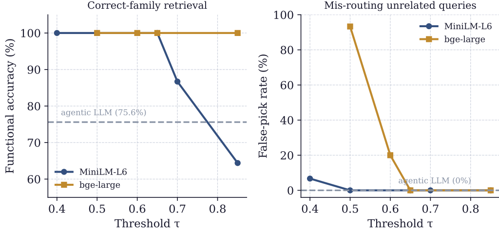
Figure 6. A plain embedding retriever matches the LLM-based selector. On the 58-program corpus, both embedding backbones reach 100% correct-family retrieval (left) at 0% mis-routing of unrelated queries (right) once the similarity threshold \tau is tuned, against the agentic selector’s 75.6% (dashed). The selector’s implementation is not load-bearing; we keep the agentic one only for its interpretable logs and tuning-free operation. Full sweep in Appendix G.
