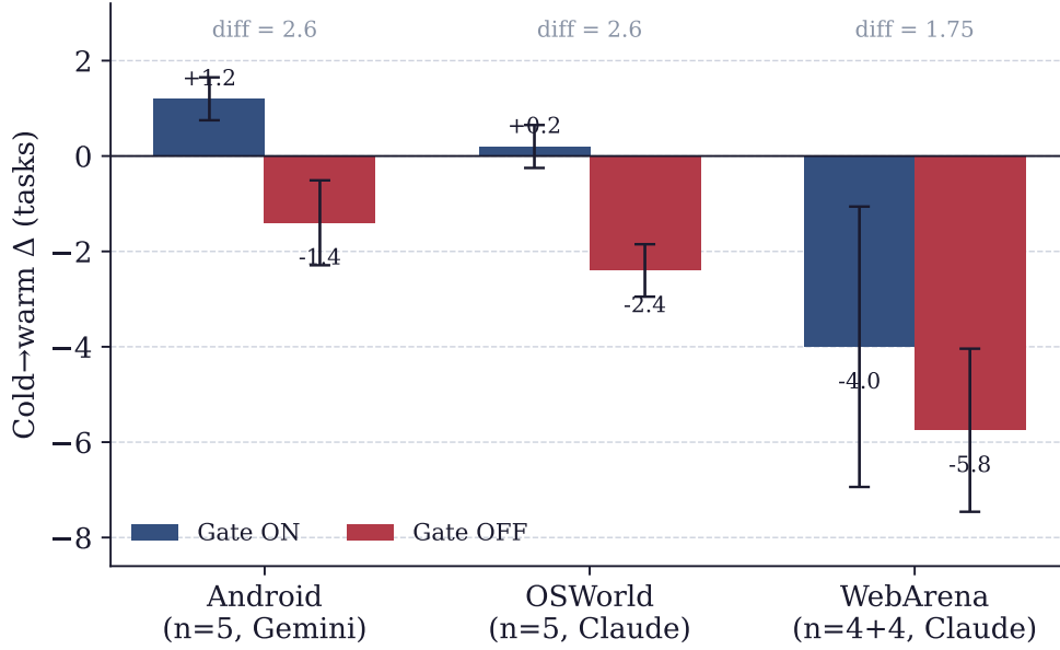
Figure 4. The gate is what makes repeated runs improve. Mean cold→warm success-rate change with the gate on (blue) versus off (red), \pm 1 s.d. On all three platforms the gate-on bar is higher: with the gate, the corpus improves the agent; without it, the corpus degrades the agent as lossy programs accumulate. The gap between the bars (the gate’s marginal value) is 1.75–2.6 tasks and points the same way everywhere—this is a property of the harness, not of any one platform. Per-seed data in Appendix C.
