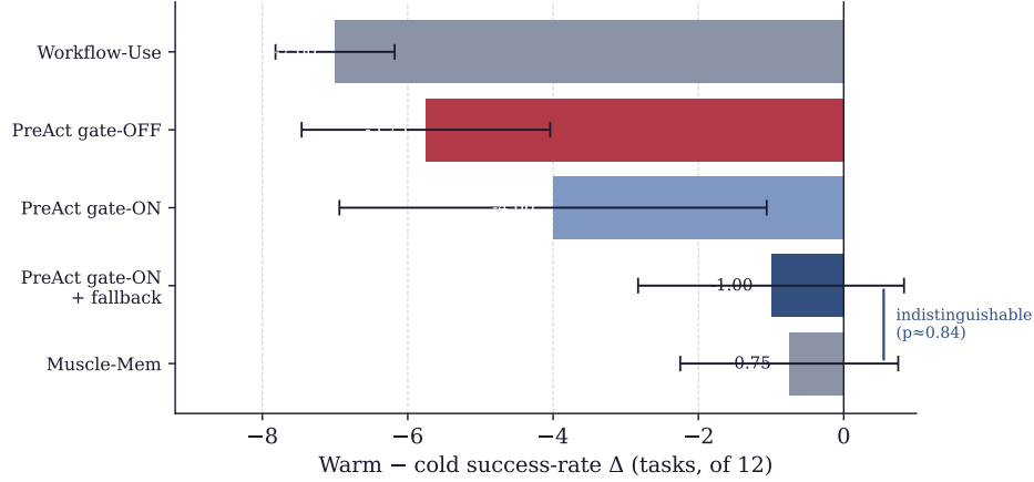
Figure 5. Closing the gap to Muscle-Mem on WebArena. Warm-cold success-rate change ( \pm 1 s.d.). As shipped, PreAct’s gate alone ( -4.0 ) trails Muscle-Mem ( -0.75 ): when the gate empties the corpus, PreAct had nothing to fall back to, whereas Muscle-Mem’s cache miss re-runs the full agent. Adding the same cache-miss fallback to PreAct ( -1.0 ) makes the two statistically indistinguishable ( p \approx 0.84 ). Workflow-Use and gate-off collapse to 0 warm, for the same reason gate-off does in Figure 4.
