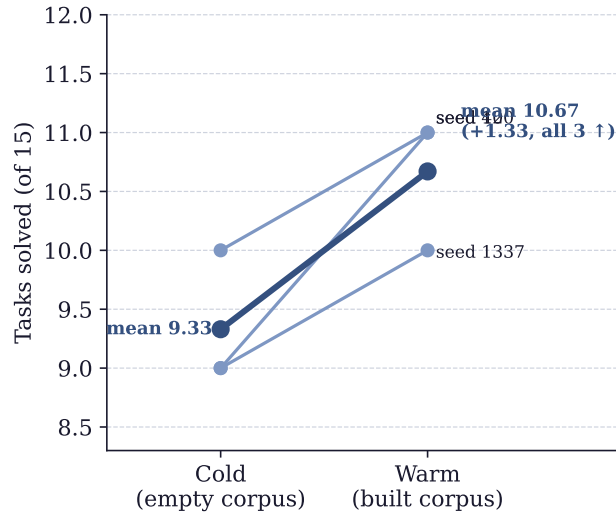
Figure 3. Cold→warm refinement is monotonic. AndroidWorld official-15 success rate, three Gemini 3 Flash seeds with the corpus reset per seed. Every seed improves (mean 9.33 → 10.67 of 15, \Delta = +1.33 ); none regresses. Per-task detail in Appendix C.
