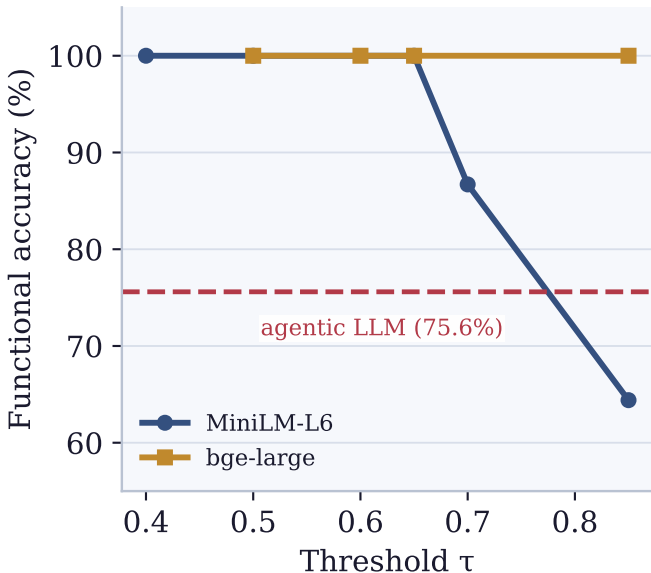
Correct-family retrieval
