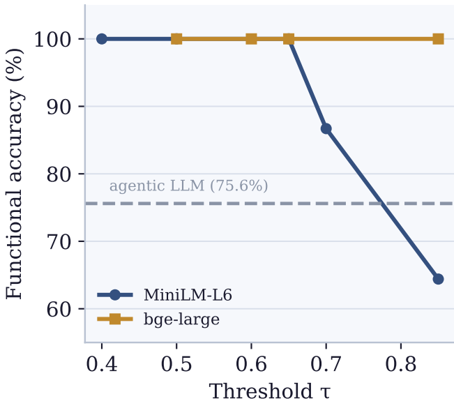
Correct-family retrieval
