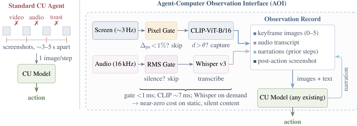
Figure 3. Standard CU agents vs. AOI-equipped agents. Left: Current agents observe through periodic screenshots ( \sim 3\text{--}5 s apart) and are blind and deaf between observations, missing video, audio, and transient UI events (X). Right: The AOI continuously monitors screen and audio streams through fast gates ( < 1 ms) that skip processing for static, silent content. When gates fire, keyframe extraction (shown here with optional CLIP filtering, see Section 6.2) and Whisper ASR produce images and text for the observation record. Visual narrations feed back as persistent text memory. The AOI wraps any existing CU model with zero retraining.
