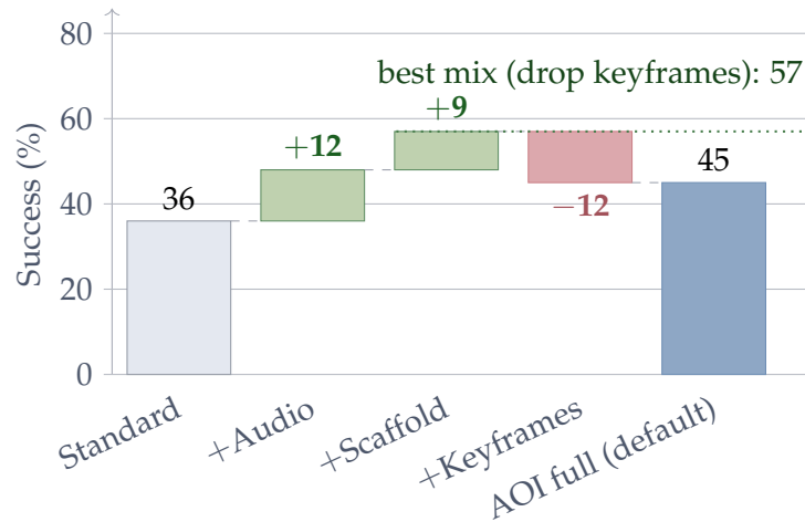
Figure 10. The AOI’s small +9 pp net on Gemini 3 Flash is a three-way cancellation, not saturation. Audio (+12) and the structured scaffold (+9) help as on every other model, but the keyframe-image stream regresses −12 pp—so the default bundle nets only 36 → 45. Dropping just the keyframes recovers 57/100 (+21 pp over Standard), showing the slack is real and the bundle merely mis-tuned. Underlying per-mode and per-family tables are in Appendix E.
