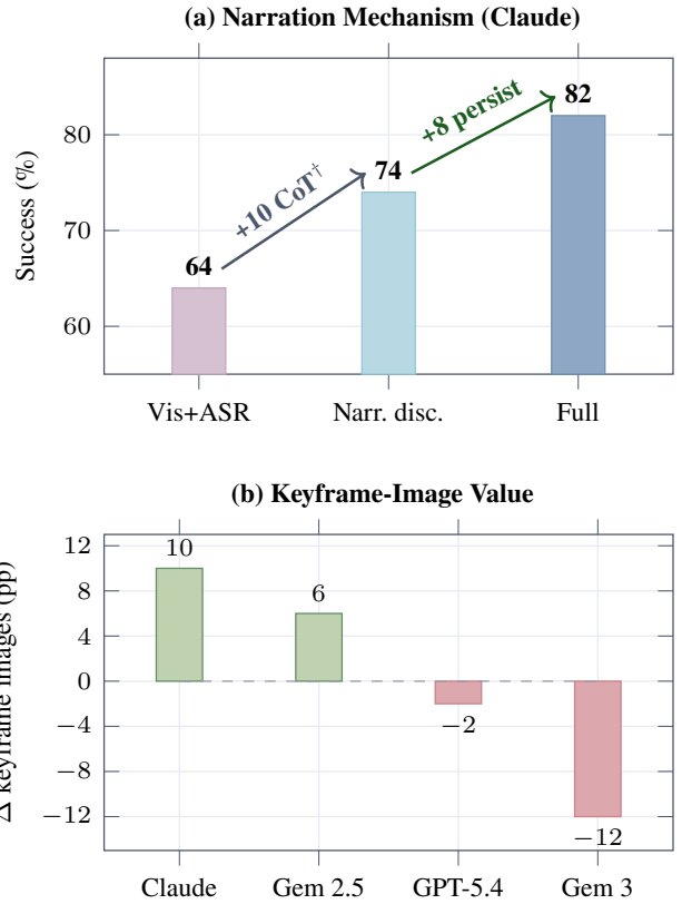
Figure 7: Contribution of narration and keyframes. (a) Visual narration improves performance, with most of the gain arising from inference-time articulation rather than persistent memory. (b) The value of keyframes is model-dependent: positive for Claude and Gemini 2.5, neutral for GPT-5.4, and negative for Gemini 3.
