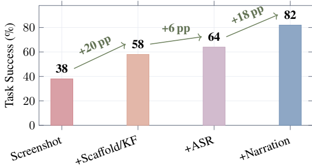
Figure 6: Progressive contribution of AOI components on Claude Sonnet 4.6.
