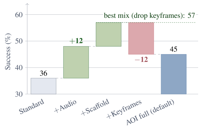
Figure 8: Gemini 3 Flash component decomposition: audio and the scaffold help, while keyframes cost 12 pp.
