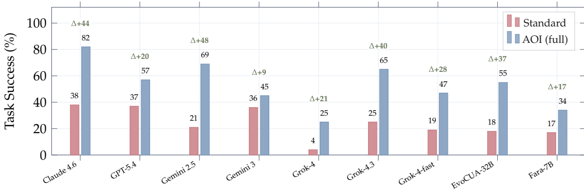
Figure 5. Main results on DynaCU-Bench (100 tasks). The AOI produces large gains across all nine CU models without any retraining; green numbers show the absolute improvement in percentage points. Gemini 2.5 Flash shows the largest gain (+48 pp) and Claude the highest absolute score (82%). Gemini 3 Flash is the lone outlier, gaining only +9 pp because its keyframe stream regresses (Section 6.6). Exact (asymmetric) 95% Wilson confidence intervals on every bar are tabulated in Table 2.
