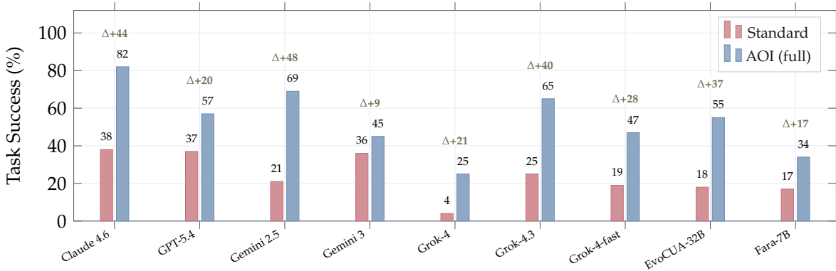
Figure 5. Main results on DynaCU-Bench (100 tasks). The AOI produces large gains across all nine CU models without any retraining; green numbers show the absolute improvement in percentage points. Gemini 2.5 Flash shows the largest gain (+48 pp) and Claude the highest absolute score (82%). Gemini 3 Flash is the lone outlier, gaining only +9 pp because its keyframe stream regresses (Section 6.6). Exact (asymmetric) 95% Wilson confidence intervals on every bar are tabulated in Table 2.
