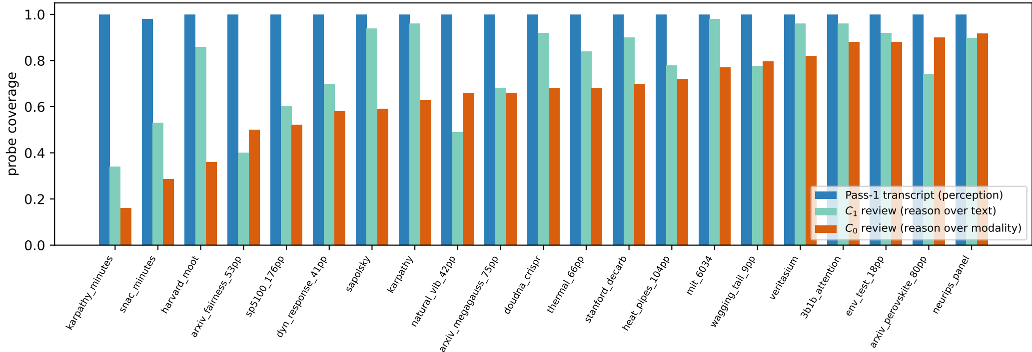
Perception check: the model perceives ~everything (Pass-1 \approx 1.0) but end-to-end reasoning drops ~35%
