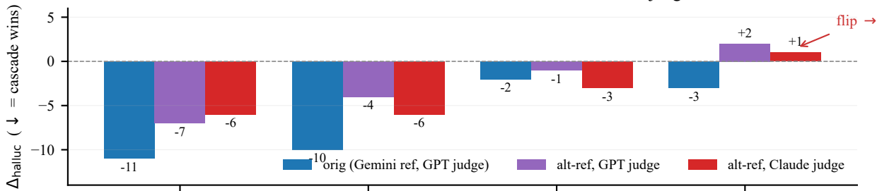
Reference-bias check: cascade direction across 4 cells under 3 ref/judge combos
