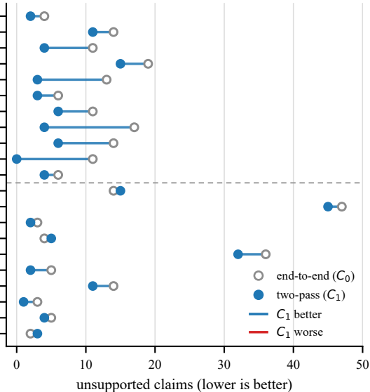
(b) Hallucinations, same cells
