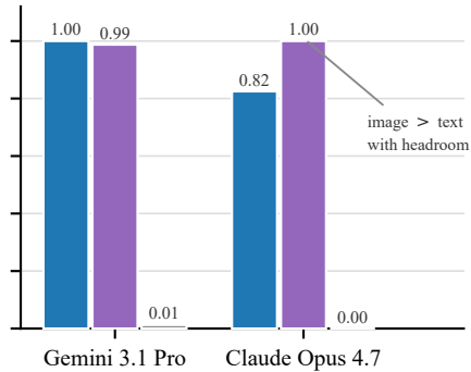
Frontier reasoning: multi-hop (sum of 6 facts)
