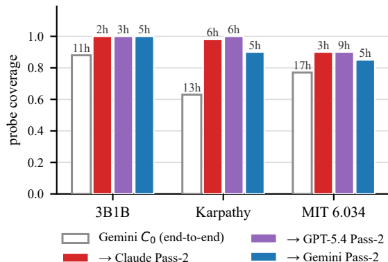
(d) gpt-audio transcript unlocks text-only models: every pipeline beats end-to-end (labels = hallucinations)
