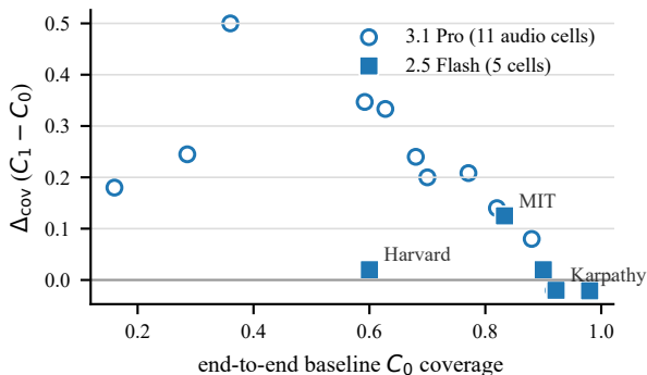
(c) Audio, two Gemini models: gain tracks headroom, not model identity
