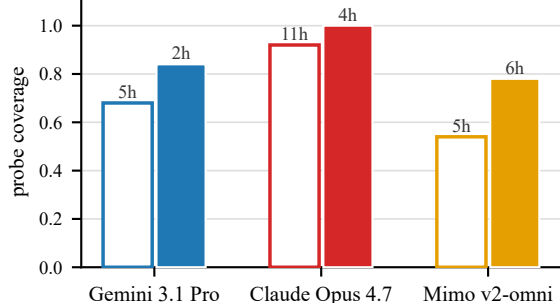
(a) Thermal 66pp: every vendor improves (open = C_0 , filled = C_1 ; labels = hallucinations)
