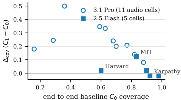
(c) Audio, two Gemini models: gain tracks headroom, not model identity
