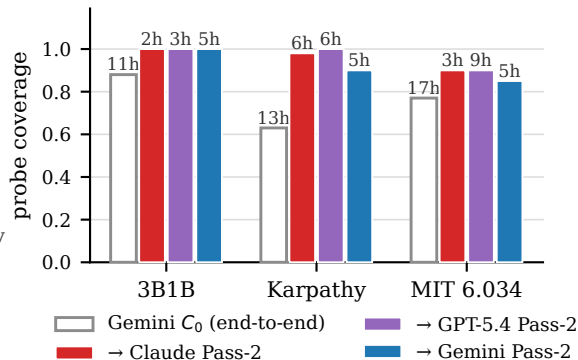
(d) gpt-audio transcript unlocks text-only models: every pipeline beats end-to-end (labels = hallucinations)
