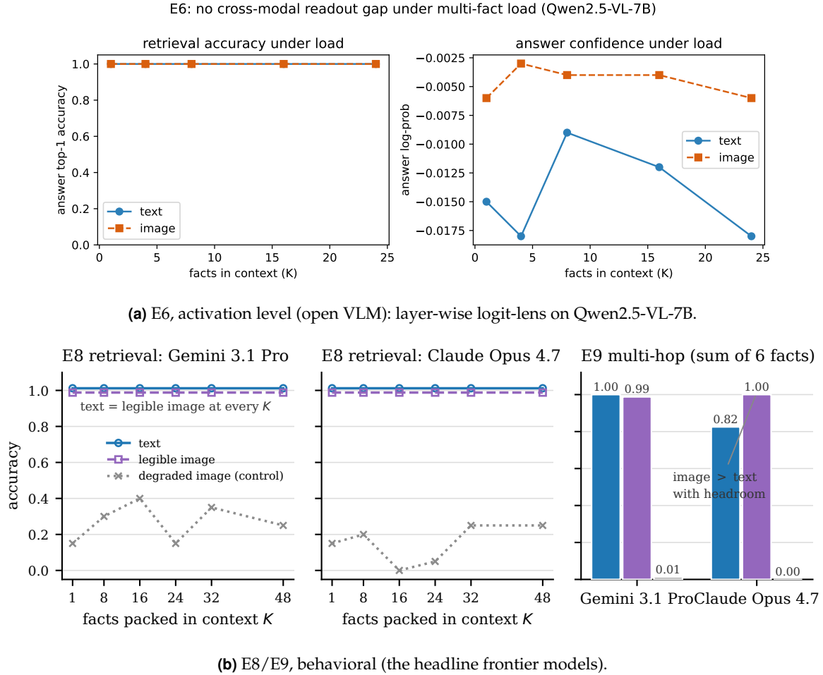
Figure 5. Text is not a better reasoning substrate than pixels (H1 is false for legible content). (a) E6: novel synthetic facts presented as text vs. as an image of that text are read with the same accuracy and the same answer-token log-prob at every load K \leq 24 ; readout depth is TOST-equivalent within \pm 1 layer (replicated on Qwen2.5-VL-3B; Appendix J). An omni-model audio analogue (E7) gives the same null once the TTS is intelligible (Appendix A). (b) The null holds behaviorally on the exact headline frontier models. E8 (left, center): single-fact retrieval from packed sets of up to K=48 novel facts is identical from text and legible image on both models (pooled gap +0.000 , TOST-equivalent within \pm 0.1 ), while a degraded low-DPI control collapses to 0.15–0.27—the probe detects gaps when they exist. E9 (right): multi-hop reasoning (sum 6 packed facts; the answer is never visible). Gemini is at ceiling in both modalities; Claude without extended thinking has headroom (text 0.825) and the image is reliably better (1.00, gap +0.175 , 95% CI [0.10, 0.26] )—the opposite of H1’s prediction.
