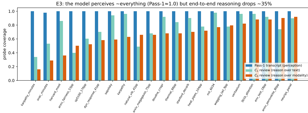
Figure 4. E3: the bottleneck is not perception. Per cell (sorted by C_0 coverage): the model’s own transcript of the source (blue) covers \approx 1.0 of probes everywhere, while the end-to-end review (orange) surfaces 0.65 on average and the two-pass synthesis (green) 0.77. Pooled, 361/362 probes the end-to-end pass drops (99.7%, Wilson 95% CI [98.5%, 99.9%]) are present in the model’s own transcript.
