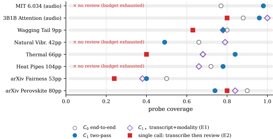
Figure 6. E2: the win needs two passes with independent output budgets; E1: removing the modality is not the engine. Probe coverage on the 8-cell condition grid (single-seed; raw counts in Appendix A, Table 5). A single call instructed to transcribe then review (red squares) collapses below the two-pass configuration on every paper that produced a review, and on three cells emits no review at all—the transcript exhausts the output budget. At n=5 seeds on all 21 cells the collapse replicates: single-call coverage sits below two-pass by \Delta_{\text{cov}} = -0.111 (bootstrap 95% CI [-0.170, -0.038] , Wilcoxon p=0.019 , mixed-effects p<10^{-3} ), with 7 runs emitting no review. Conversely, giving the synthesis pass the transcript and the raw modality ( C_{1+} , open diamonds) preserves and sometimes maximizes coverage; at n=5 on all 21 cells it shifts coverage by only +0.069 (CI [-0.001, +0.154] , inconclusive) while re-adding hallucinations on 14/21 cells—the Mode-B effect of §5.
