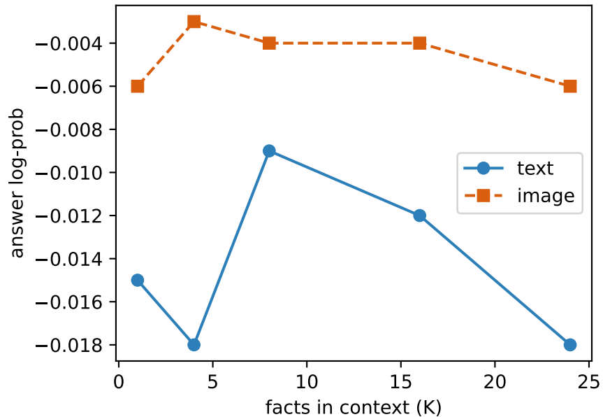
answer confidence under load
