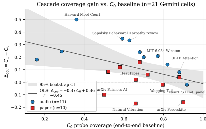
Figure 7. The inverse-baseline law. Cells with weaker end-to-end coverage gain more from decomposition. Circles denote audio and squares papers; the line and band are OLS and its bootstrap CI. Counter-cells have little headroom or exhibit Modes A/B.
