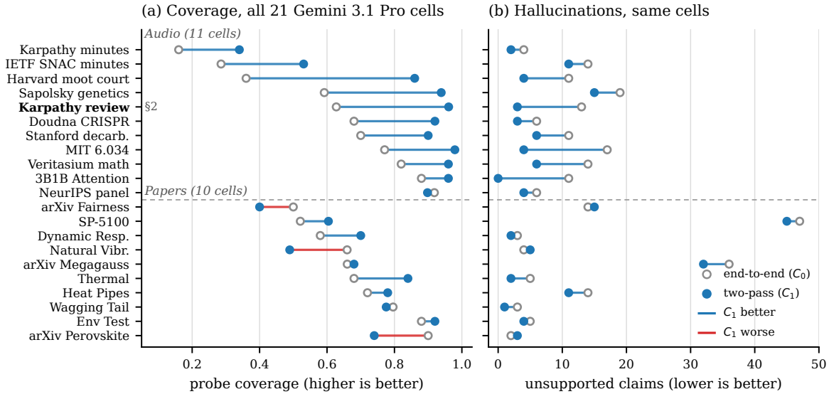
Figure 8. Per-cell results for all 21 Gemini 3.1 Pro cells. Cells are sorted by C_0 coverage within modality; the bold row is the running example. C_1 improves coverage and reduces unsupported claims on most cells; red connectors mark regressions.
