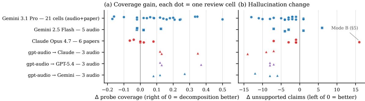
Figure 1. Two-pass decomposition improves long-form review. Each dot is one cell’s change from end-to-end ( C_0 ) to transcribe-then-review ( C_1 ): (a) probe coverage and (b) unsupported claims. Rows use the same weights; gpt-audio rows are mixed pipelines.
