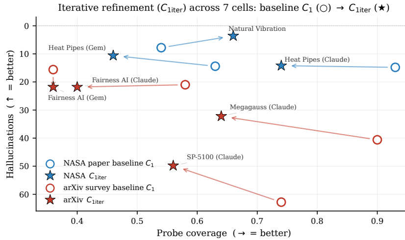
Figure 13. Quote-grounded iterative refinement ( C_{1iter} ) across seven cells ( n=5 means). Stars show C_{1iter} relative to plain C_1 (open circles). Natural Vibration is the only clean Pareto win; other cells trade coverage against faithfulness or regress, depending on whether Mode B is the binding constraint.
