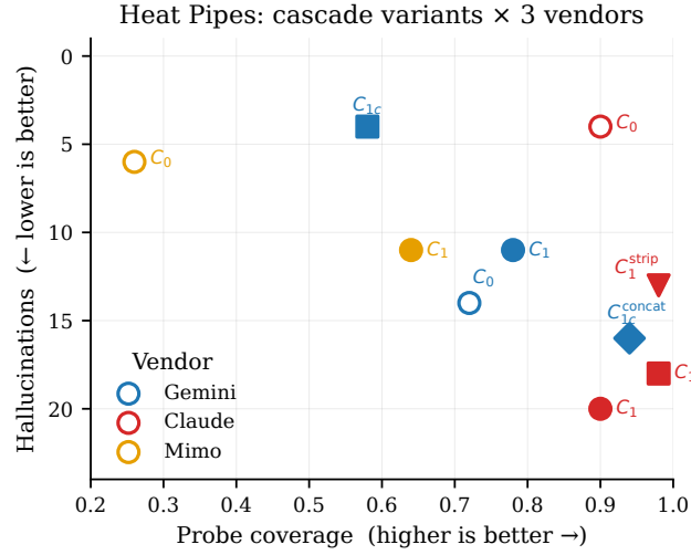
Figure 12. Heat Pipes Pareto frontier across vendors and cascade variants. The Gemini cascade is small-Pareto-positive; Claude C_1 regresses on faithfulness, leaving C_0 on the Pareto frontier (the Mode-B signature); MIMO trades faithfulness for coverage (Modes A+B compounded).
