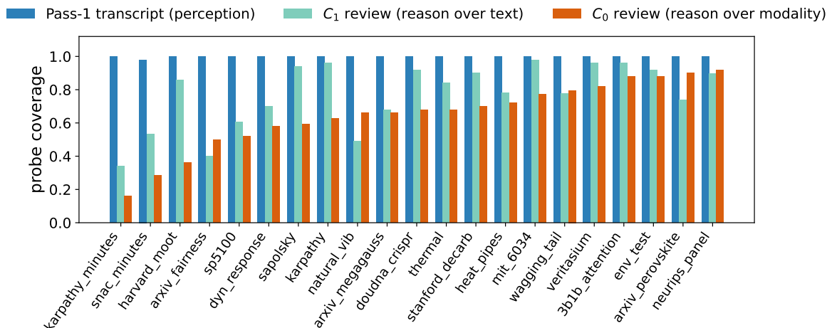
Figure 4. Perception check. Per cell, the model’s own transcript (blue) covers nearly all probes—far more than either the end-to-end (C 0 , orange) or two-pass (C 1 , green) review. Almost all content the end-to-end pass drops is present in that transcript.
