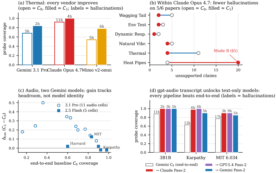
Figure 9. Cross-model results follow the inverse-baseline law rather than replicating uniformly. (a) On Thermal, all three vendors gain coverage. (b) In Claude’s feasible NASA cells, hallucinations fall on all but Heat Pipes (Mode B), while short papers have little coverage headroom. (c) Flash’s strong audio baseline leaves gains only on MIT and Harvard; Karpathy regresses. (d) Mixed pipelines let text-only models review audio and beat the native end-to-end baseline on both axes.
