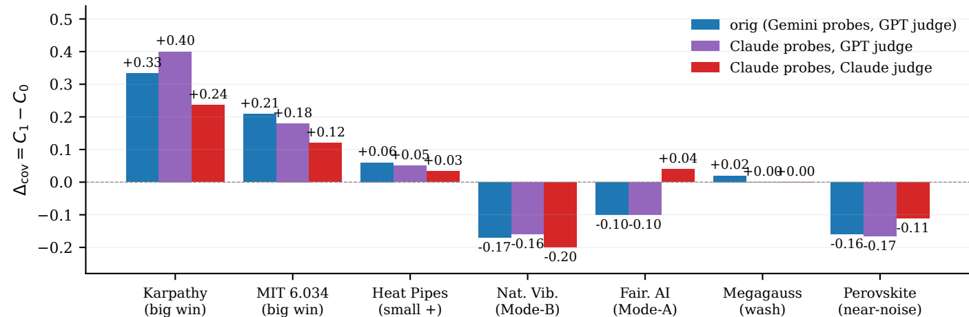
Probe-circularity check across 7 cells \times 2 judges (revised)
