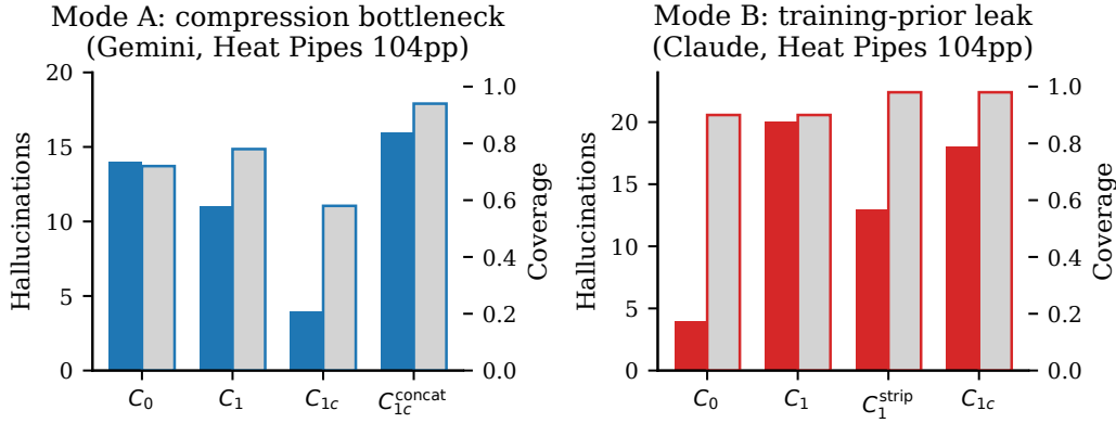
Figure 4: Two cascade failure modes on Heat Pipes 104pp. Left: Mode A (Gemini) — Pass-2 must compress 22k→1.8k words; chunked Pass-2 ( C_{1c}^{\text{concat}} ) relieves the bottleneck and lifts coverage from 0.78 to 0.94 at a +5-hallucination cost (11→16), a Pareto move along the frontier rather than strictly above it. Right: Mode B (Claude) — C_1 hallucinates 5× more than C_0 ; replacing citation surface forms (Reference N) with neutral placeholders ( C_1^{\text{strip}} ) reduces hallucinations 20→13. Hallucinations on left axis (lower better); coverage on right axis (higher better).
