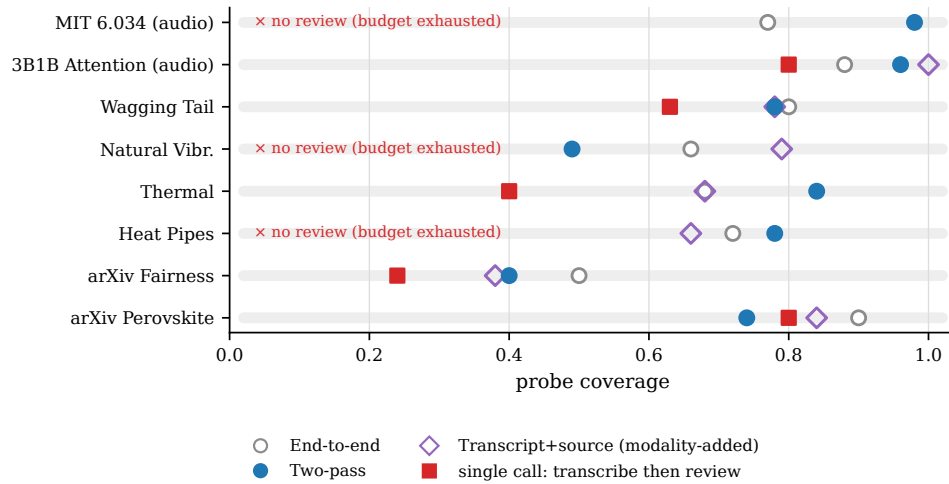
Figure 6. The benefit requires two output budgets, not removal of the modality. On the 8-cell grid, a one-call “transcribe then review” prompt (red squares) usually underperforms transcribe-then-review and sometimes emits no review. Adding the raw modality back to Pass 2 (the transcript-plus-source control; diamonds) does not restore the coverage benefit and adds unsupported claims.
