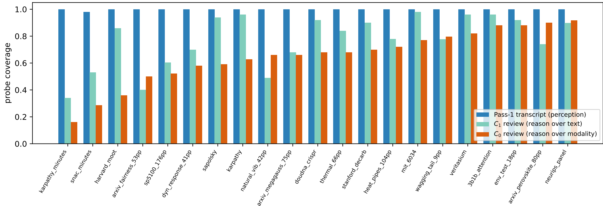
E3: the model perceives ~everything (Pass-1 \approx 1.0) but end-to-end reasoning drops ~35%
