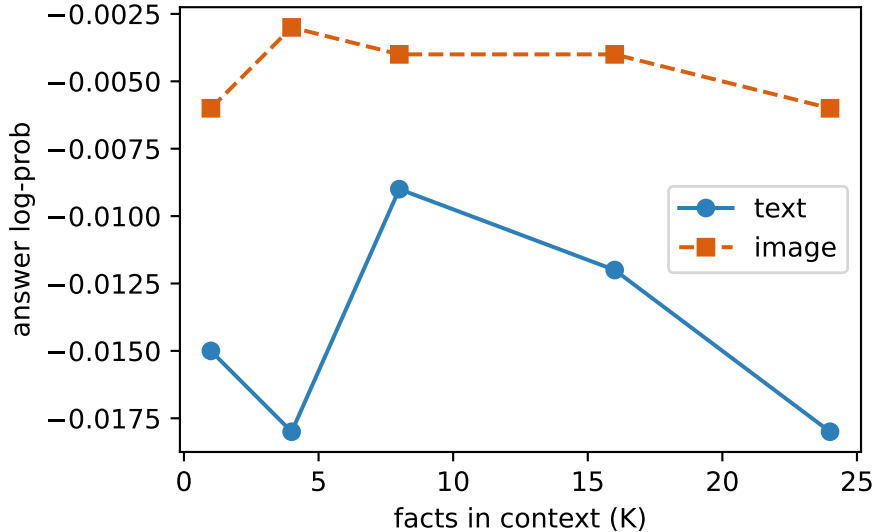
answer confidence under load
