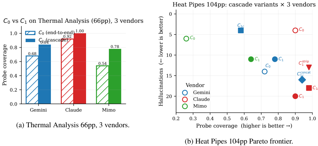
Figure 9: (a) On Thermal Analysis the cascade improves coverage on every vendor: Gemini 0.68 → 0.84, Claude 0.92 → 1.00, MIMO 0.54 → 0.78. (b) On Heat Pipes 104pp the three vendors give three patterns. Gemini cascade is small-Pareto-positive; Claude C_1 regresses on faithfulness (4h→20h) leaving C_0 on the Pareto frontier; MIMO trades +5 halluc for +38pp coverage.
